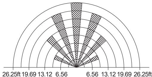
Max Horizontal detection range
