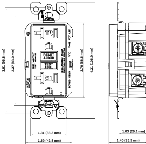
20A SmartlockPro® Self-Test GFCI
