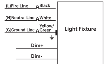
Wiring diagram
